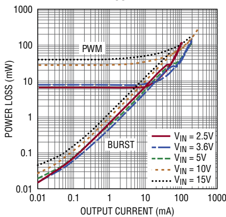
Power Loss, V_{OUT} = 3.3\text{V}
