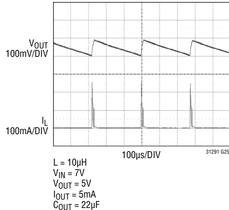
Burst Mode Ripple on V_{OUT}
