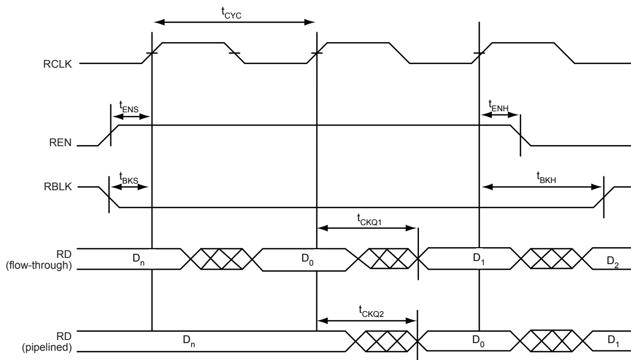
Figure 2-47 • FIFO Read
