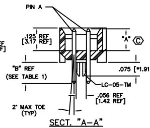
SECT. "A-A"
