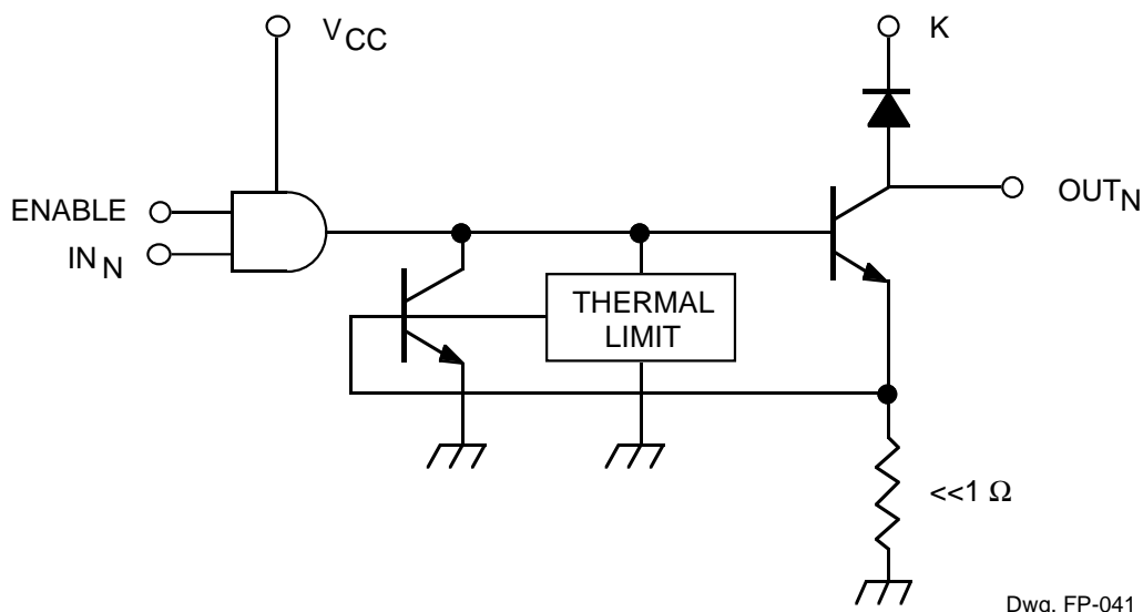
FUNCTIONAL BLOCK DIAGRAM (1 OF 4 CHANNELS)
