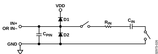
Figure 27. Equivalent Analog Input Circuit
