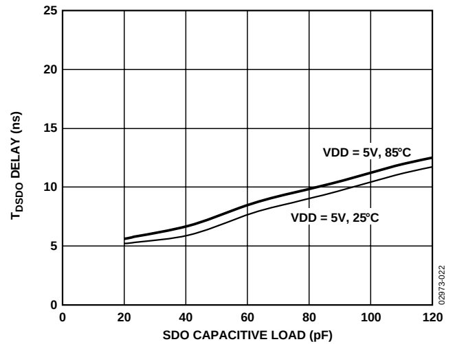
Figure 23. t_{\text{SDO}} Delay vs. Capacitance Load and Supply
