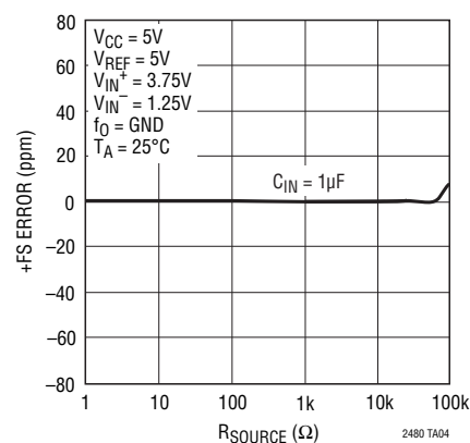
+FS Error vs R_{\text{SOURCE}} at \text{IN}^{+} and \text{IN}^{-}
