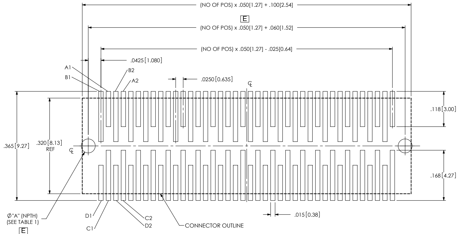
FIG 1 (-20 POSITION SHOWN) ALL DIMENSIONS ARE SYMMETRICAL ABOUT THE CENTERLINE
