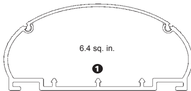
Base and Cover with No Devices
