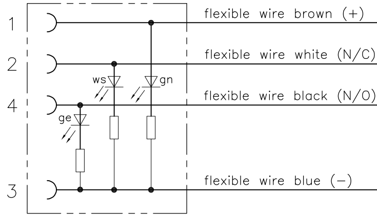
Schematic diagram
