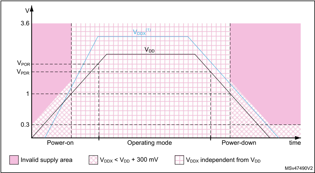
Figure 2. Power-up/down sequence
