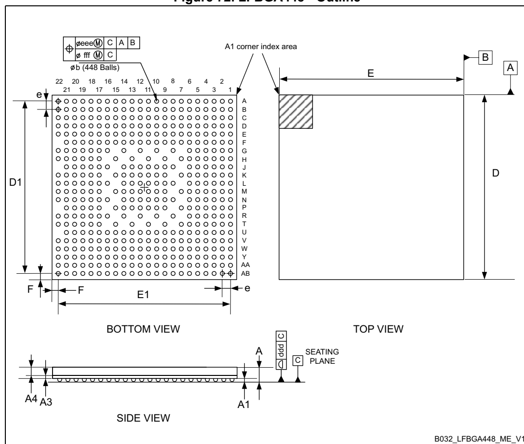
Figure 72. LFBGA448 - Outline
