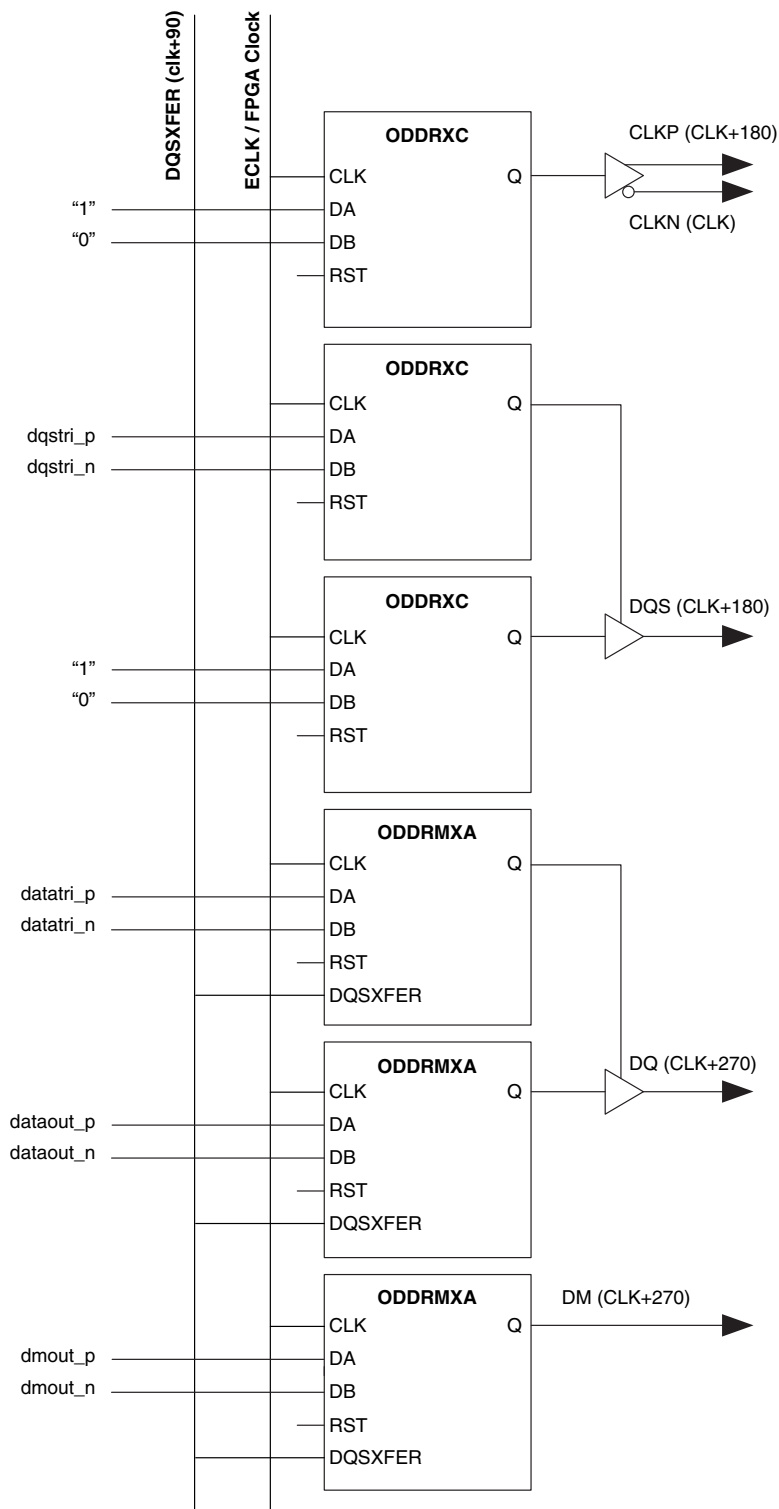
Figure 12-24. Software Implementation for Memory Write
