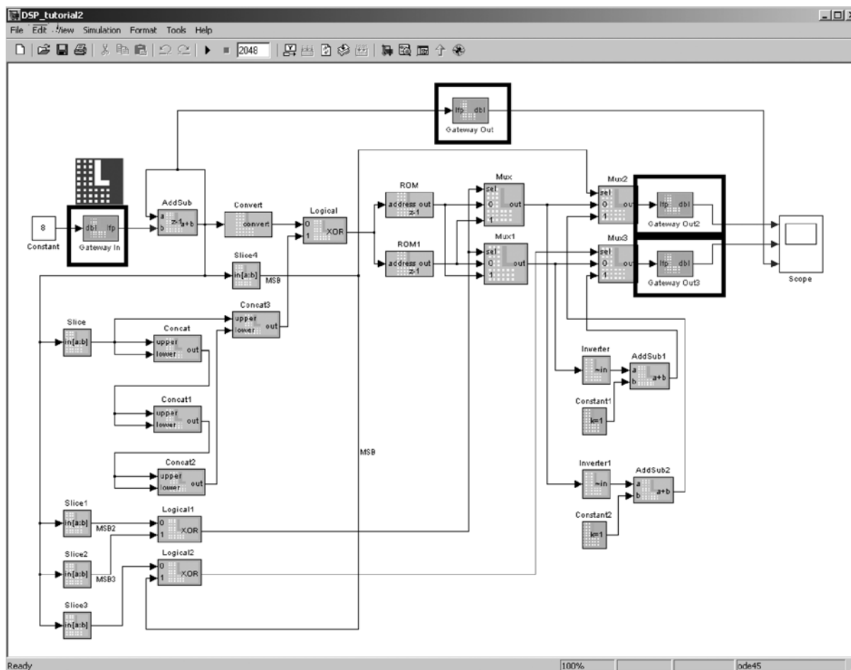
Figure 14-13. Simulink Design
