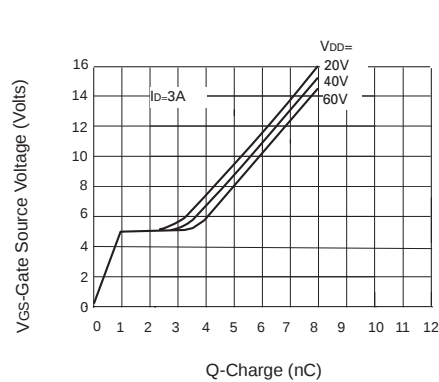
Gate charge v gate-source voltage
