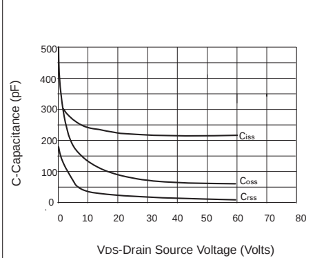
Capacitance v drain-source voltage
