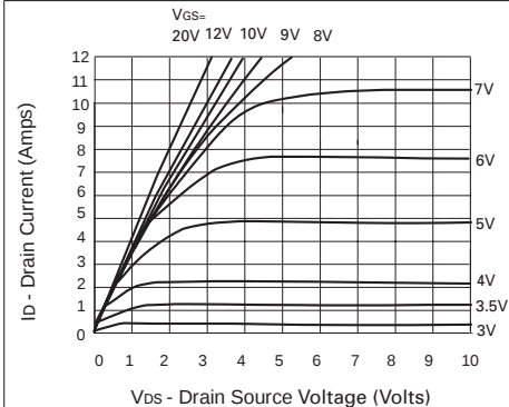
Saturation Characteristics
