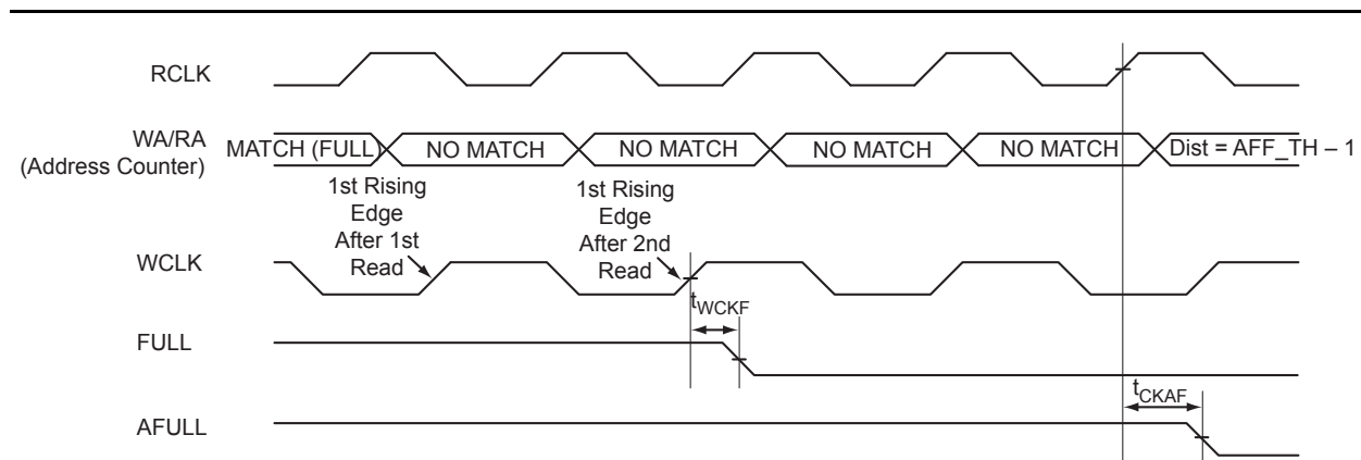
Figure 2-40 • FIFO FULL Flag and AFULL Flag Deassertion
