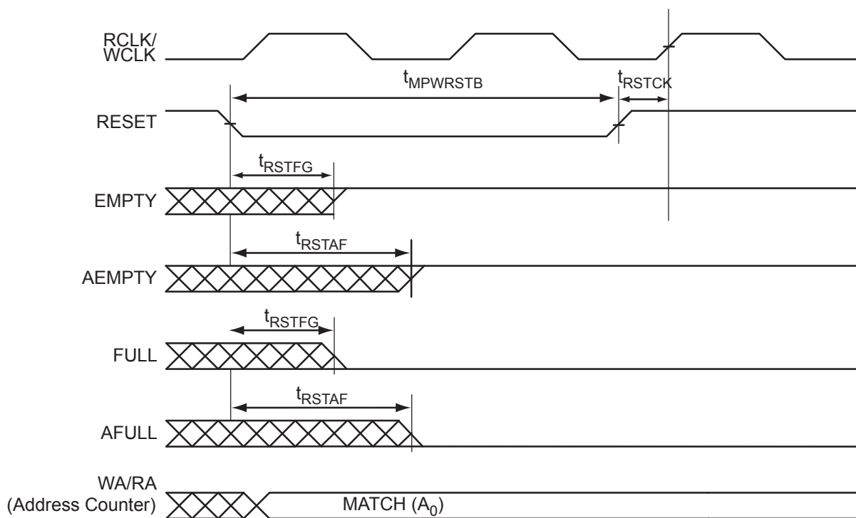
Figure 2-36 • FIFO Reset
