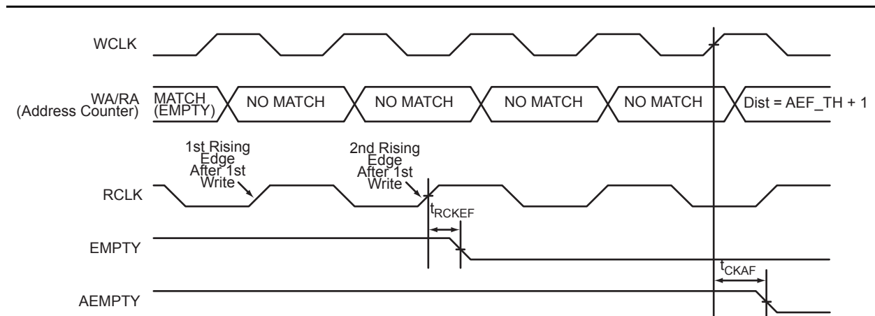
Figure 2-39 • FIFO EMPTY Flag and AEMPTY Flag Deassertion
