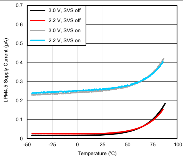
Figure 8-5. LPM4.5 Supply Current vs Temperature (LPM4.5)
