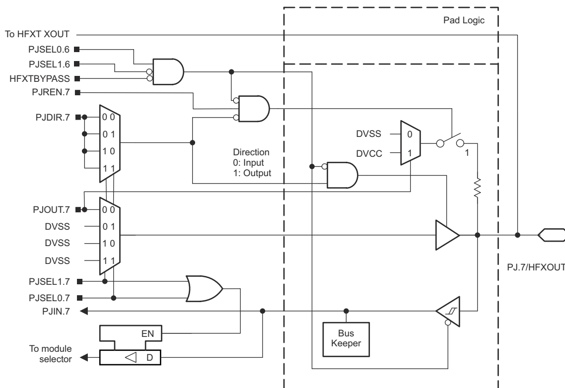
Figure 9-29. Port PJ (PJ.7) Diagram
