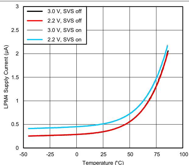
Figure 8-3. LPM4 Supply Current vs Temperature (LPM4,SVS)
