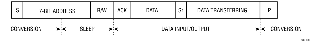
Figure 5. The LTC2481 Conversion Sequence
