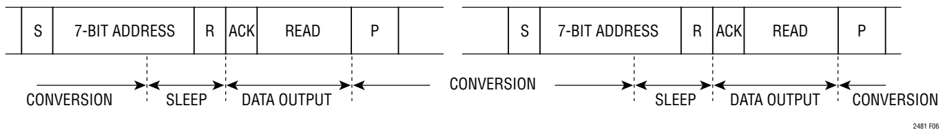
Figure 6. Consecutive Reading at the Same Configuration
