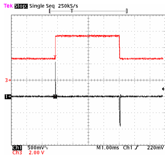
FIGURE 60. LINE TRANSIENT RESPONSE, 1nF LOAD
