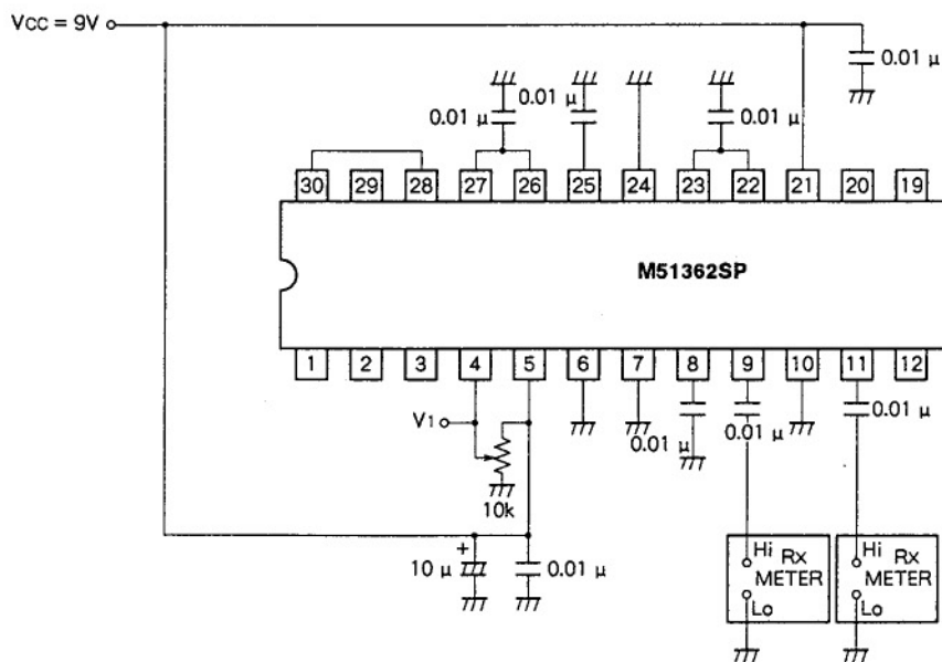
TEST CIRCUIT 2
