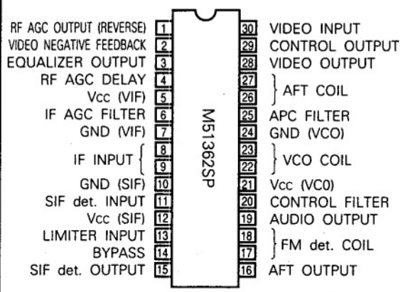
Outline 30P4B
