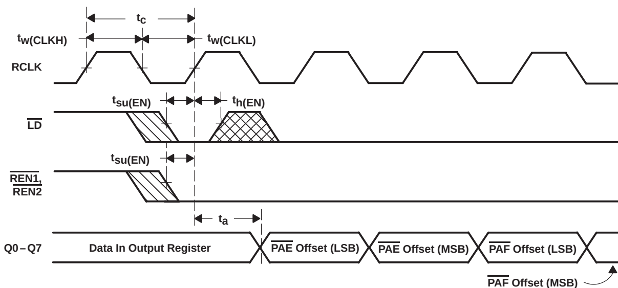
Figure 11. Read-Offset-Registers Timing
