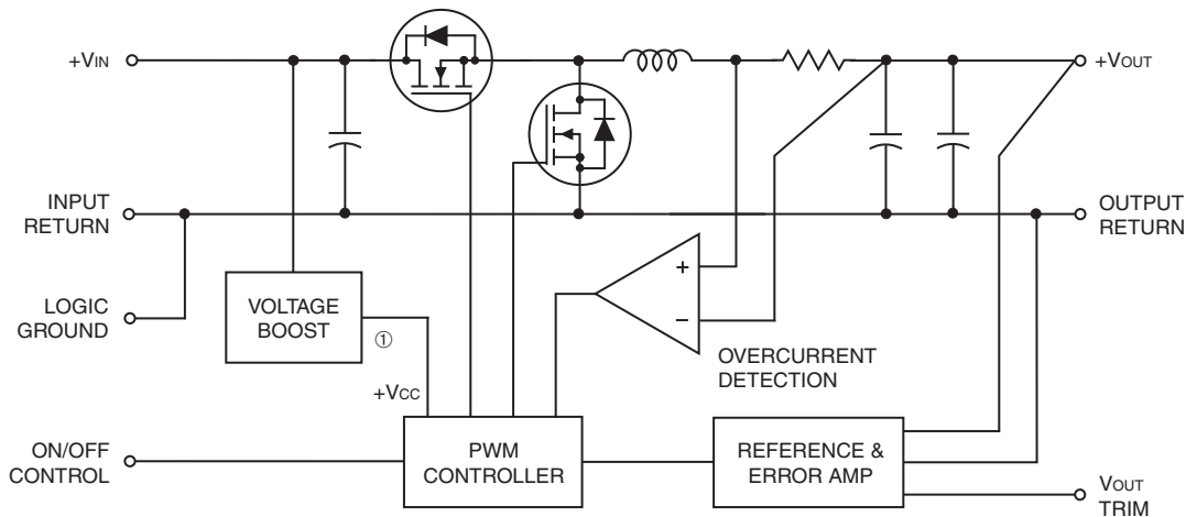
Figure 1. Simplified Schematic
