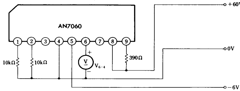
Test Circuit 5 ( V_{6-4(2)} )
