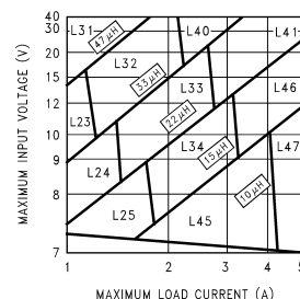
Figure 22. LM2677-5.0
