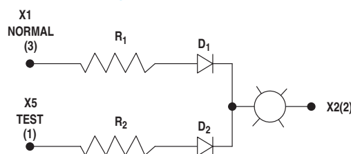
Dual Input Pilot Light Typical Application Wiring Diagram
