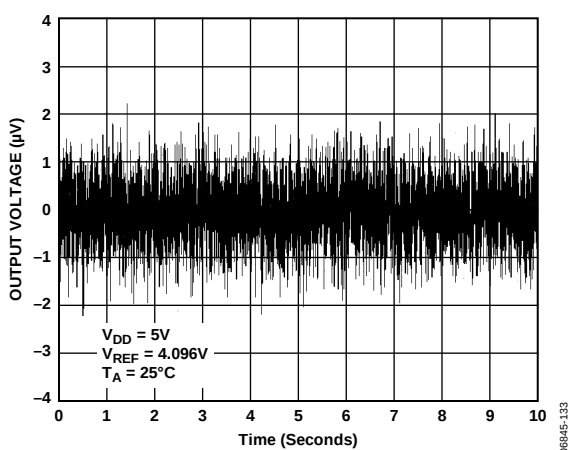
Figure 33. 1/f Noise
