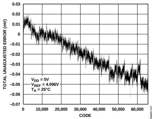
Figure 6. Total Unadjusted Error vs. Code
