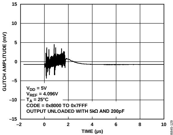
Figure 29. Glitch
