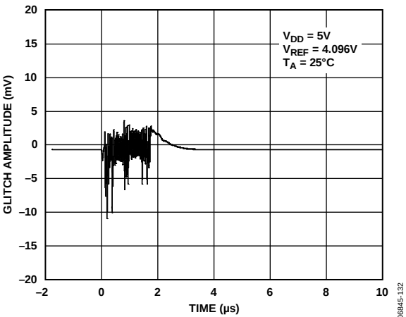
Figure 32. DAC-to-DAC Crosstalk
