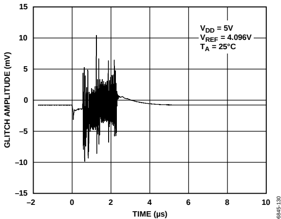
Figure 30. Analog Crosstalk
