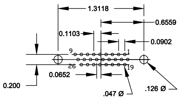
26 POSITION FEMALE
