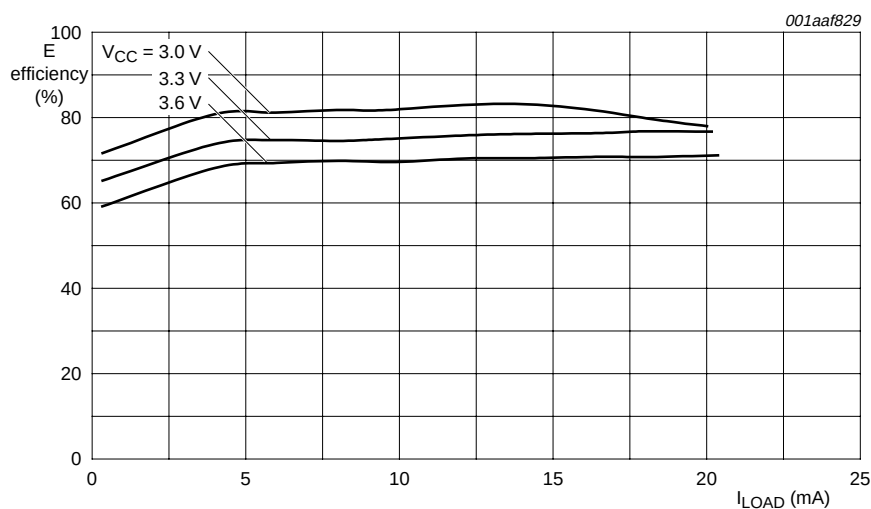
Fig 28. Efficiency as a function of load current
