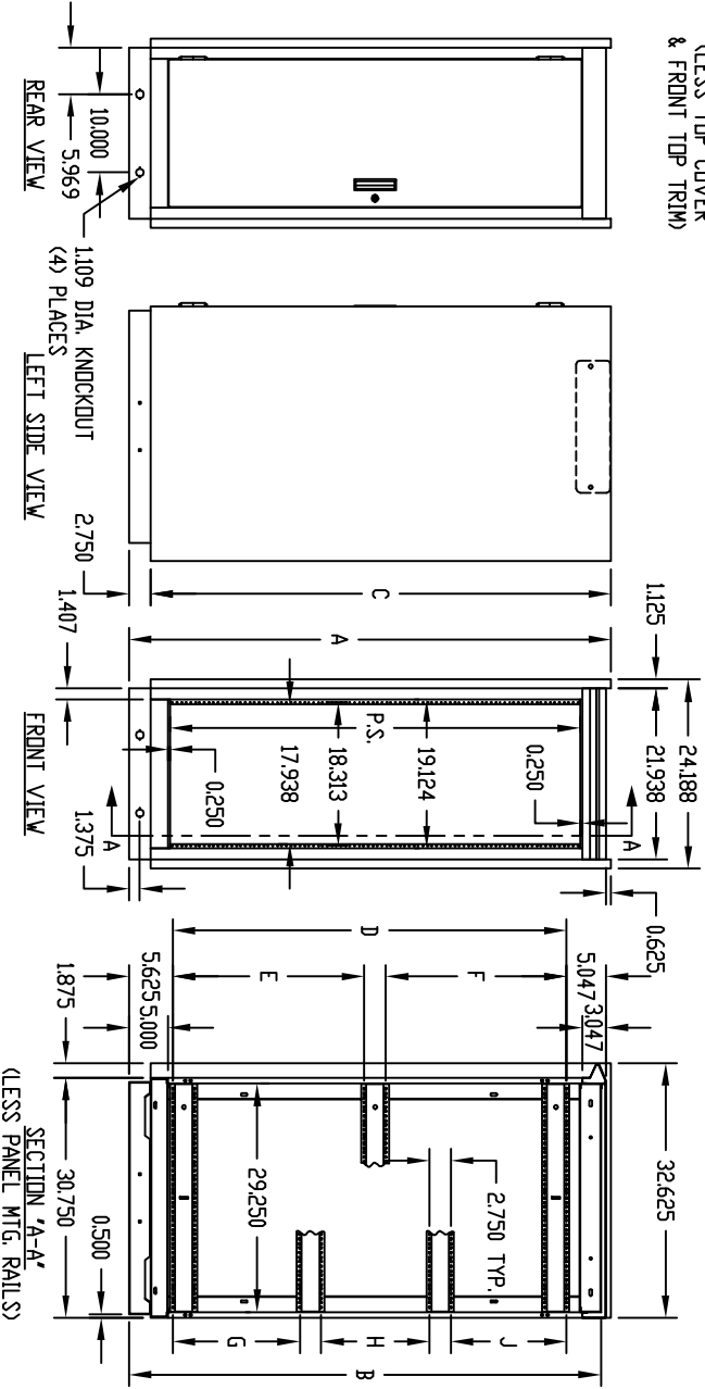
TOP VIEW
