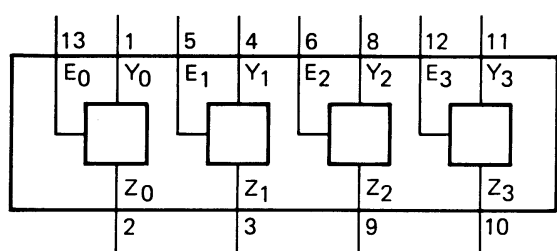
Fig.1 Functional diagram.
