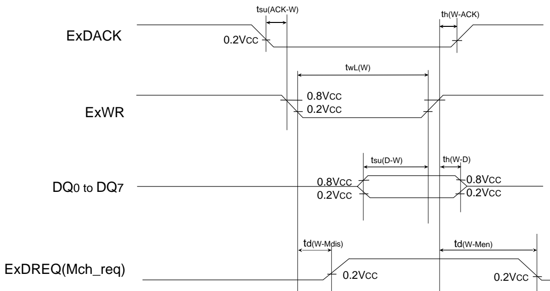
Fig. 147 Timing chart (4)
