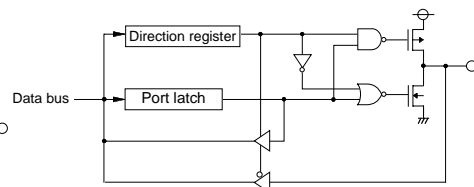
(13) Ports P53–P57
