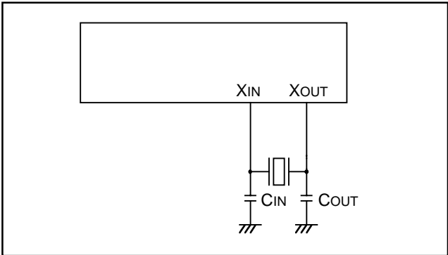
Fig. 111 Ceramic resonator or quartz-crystal oscillator circuit
