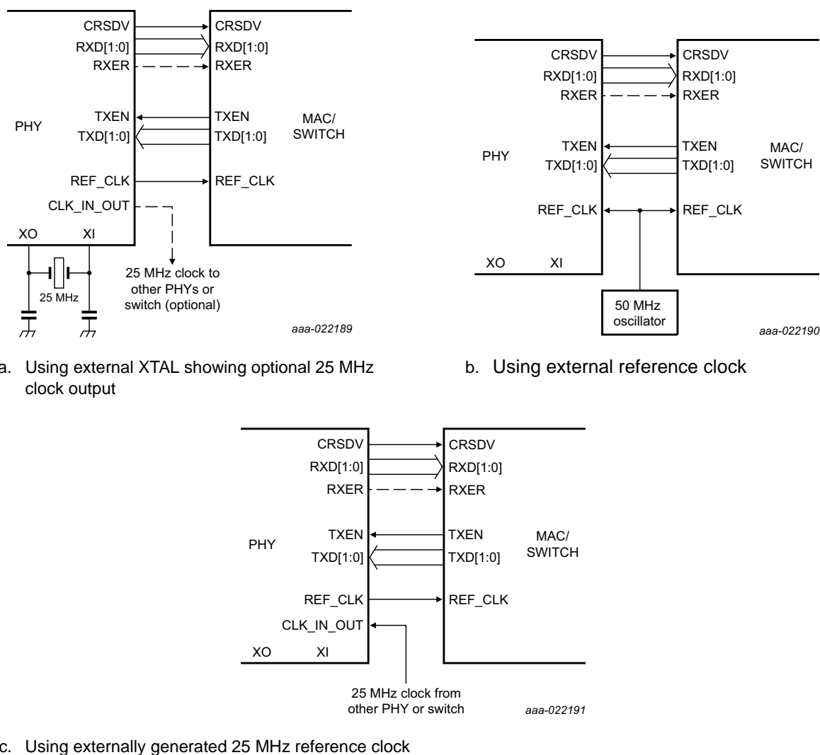
Fig 5. RMII signaling
