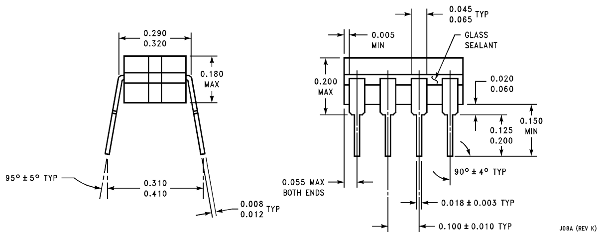
Ceramic Dual-In-Line Package NS Package Number J08A
