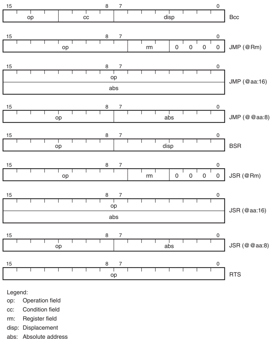
Figure 2.9 Instruction Formats of Branch Instructions
