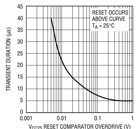
V_{CC25} Transient Immunity (LTC1326-2.5)
