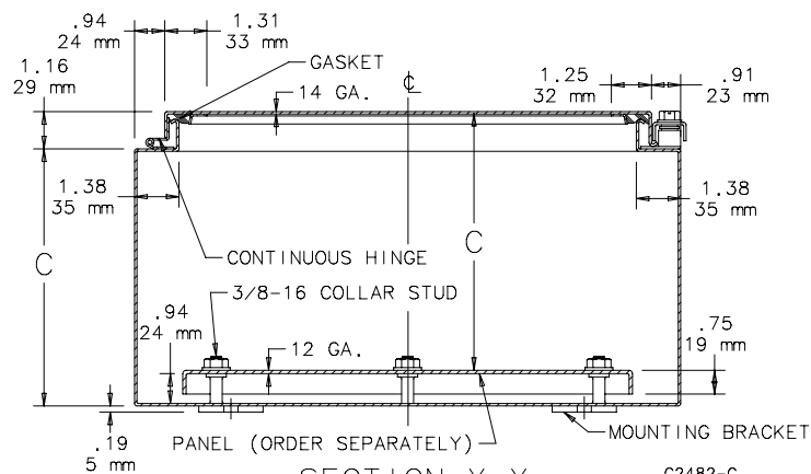
SECTION X-X
