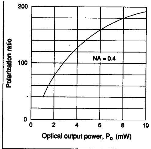
Figure 9 Optical Output Power Dependence of Polarization Ratio
