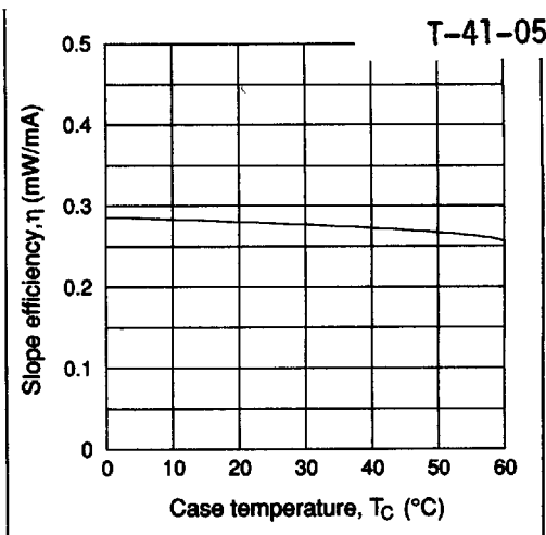
Figure 6 Temperature Dependence of Slope Efficiency
