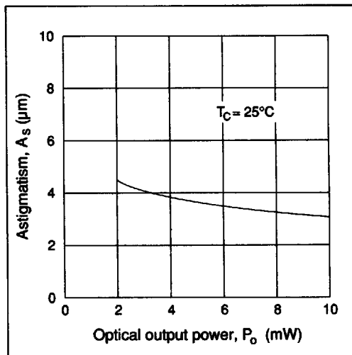
Figure 8 Optical Output Power Dependence of Astigmatism
