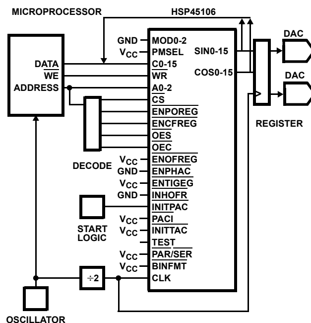
FIGURE 4. CIRCUIT FOR READING PHASE ACCUMULATOR OF NCO16 WHILE GENERATING SINUSOID
