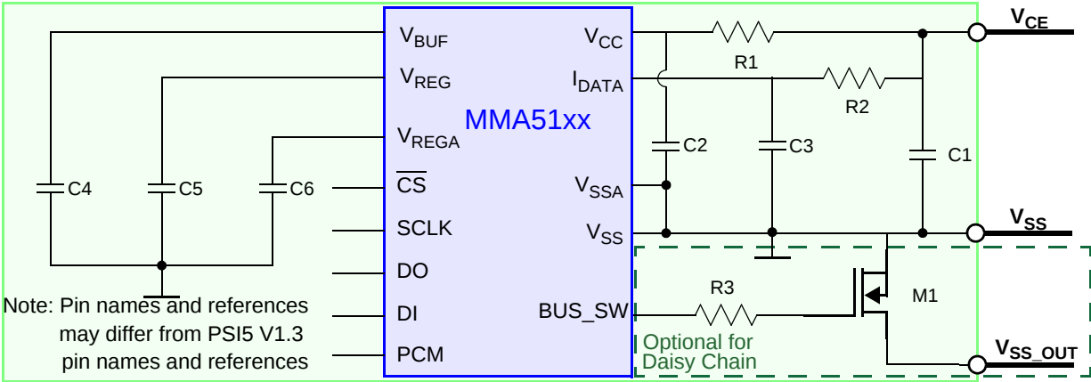
Figure 1. Application Diagram
