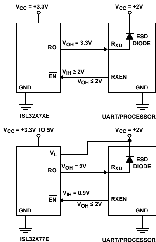
FIGURE 9. USING V I PIN TO ADJUST LOGIC LEVELS
