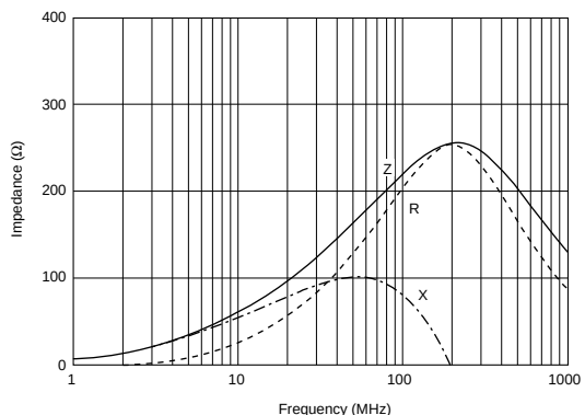
BLM21AG221SN1
