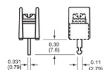
06 Handwired
