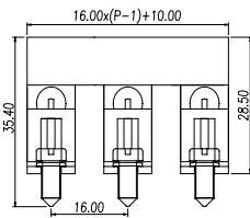
Dimensions - mm
