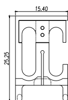
Dimensions - mm
