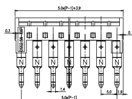
Dimensions - mm
