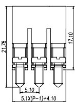
Dimensions - mm
