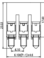
Dimensions - mm
