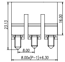
Dimensions - mm
