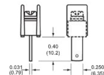
09 0.250" QC short
