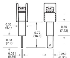
19 0.250" QC long
