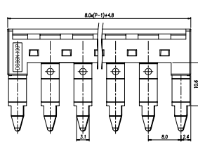
Dimensions - mm
