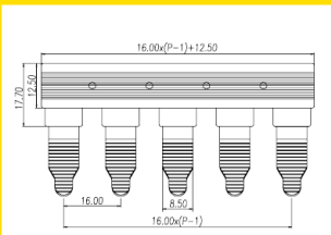
Dimensions - mm
