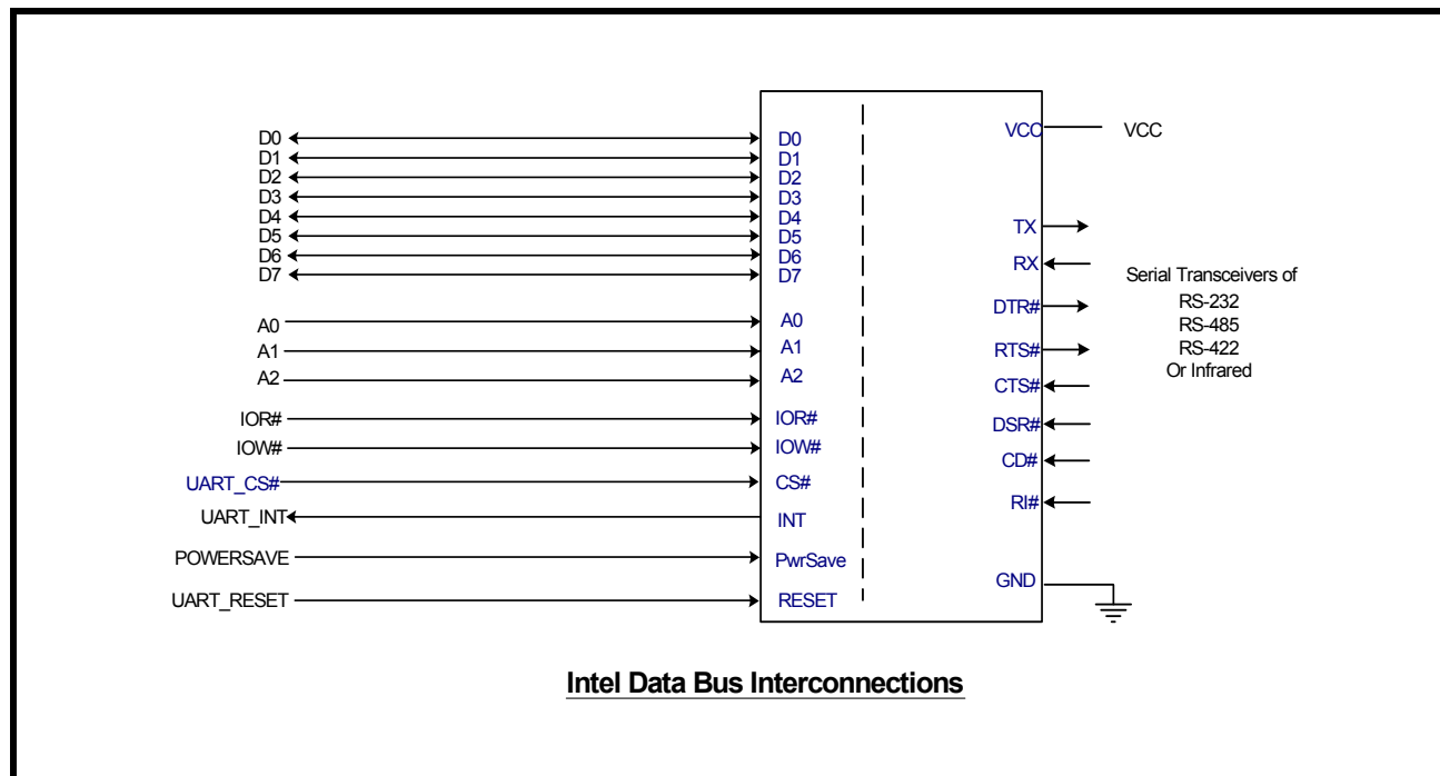
FIGURE 3. XR16M670 TYPICAL INTEL DATA BUS INTERCONNECTIONS
