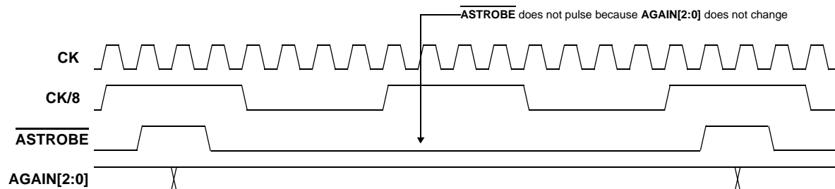
Figure 34. Timing diagram for AGC/DVGA interface, Channel A. Refer to Figure 8 for detailed timing information.
