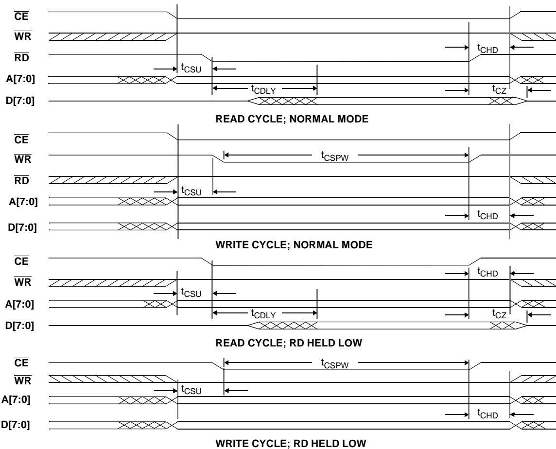
Figure 14. CLC5903 Control I/O Timing
