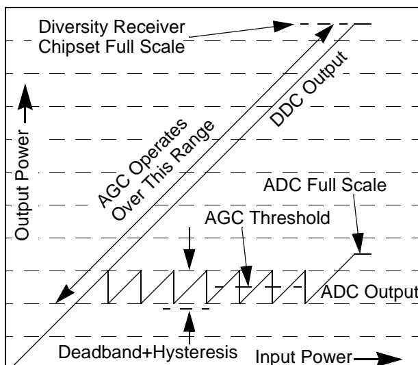
Figure 31. Output Gain Scaling vs. Input Signal
