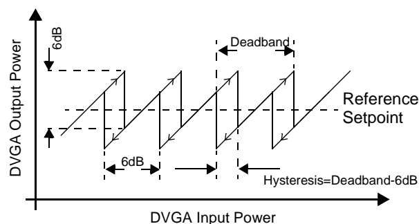
Figure 32. AGC Setup.
