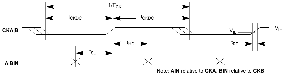
Figure 6. CLC5903 ADC Input and Clock Timing
