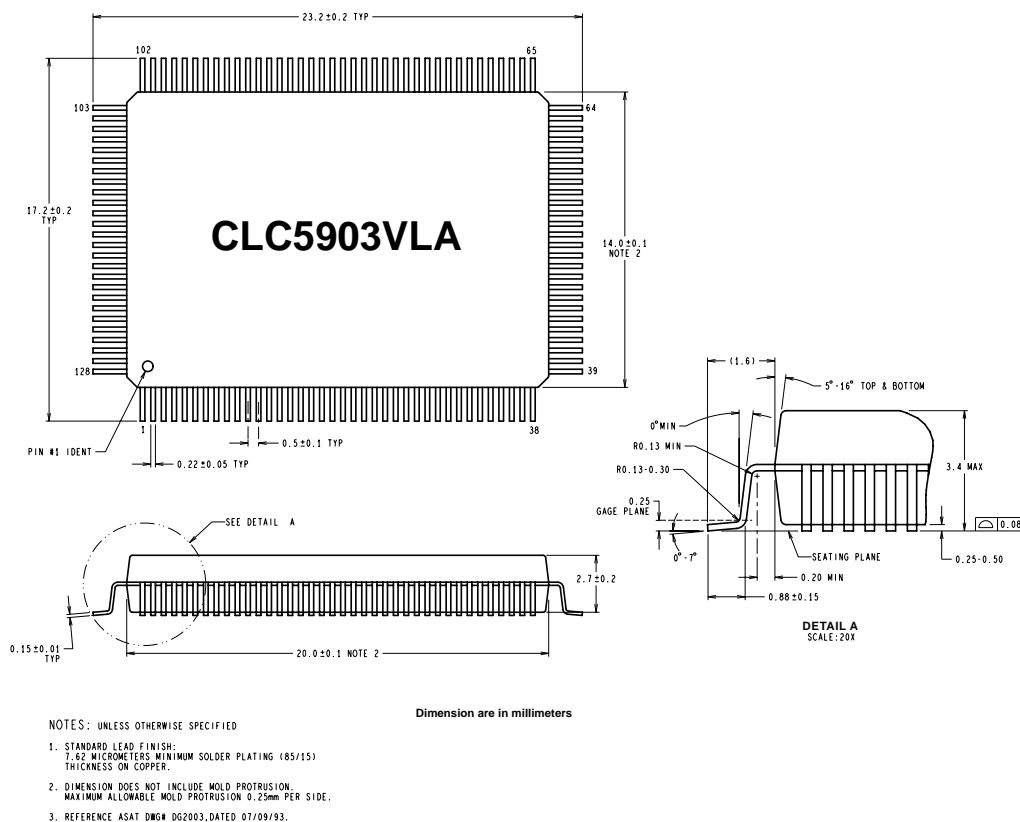
Figure 38. CLC5903VLA PQFP Package Dimensions
