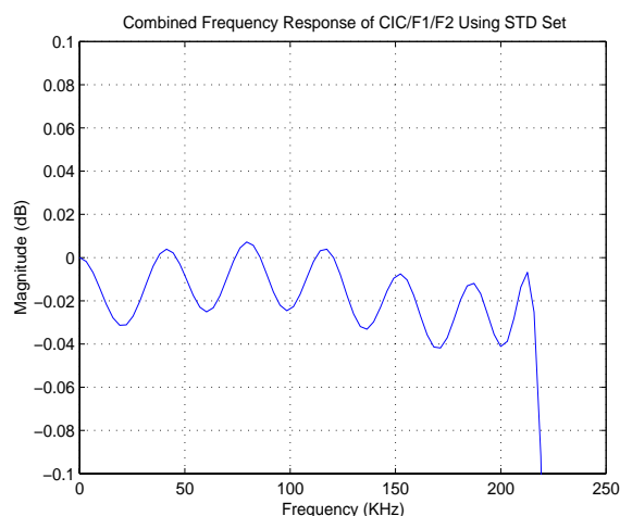
Figure 25. CIC, F1, & F2 STD Passband Flatness
