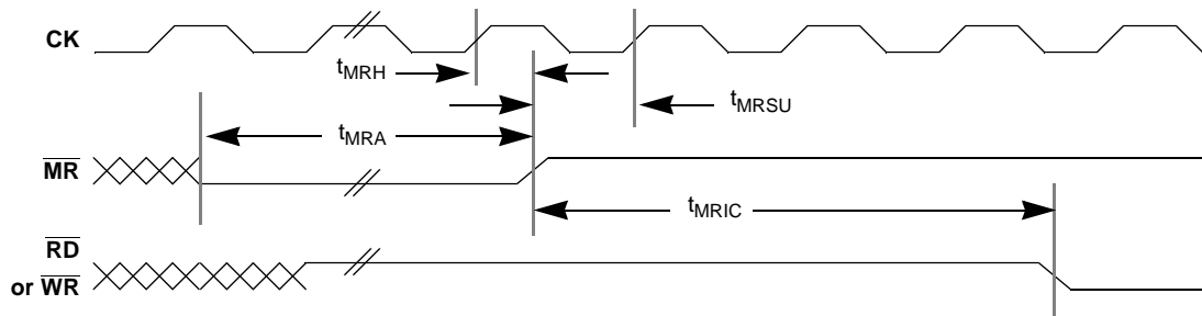
Figure 4. CLC5903 Master Reset Timing
