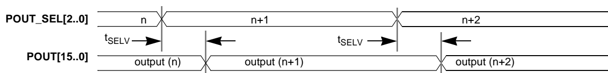
Figure 11. CLC5903 Parallel Output Select Timing
