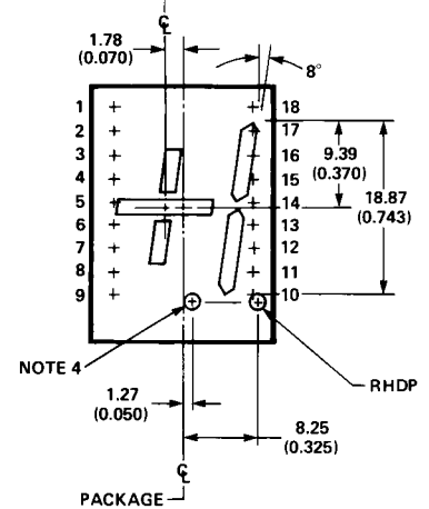
FRONT VIEW E
