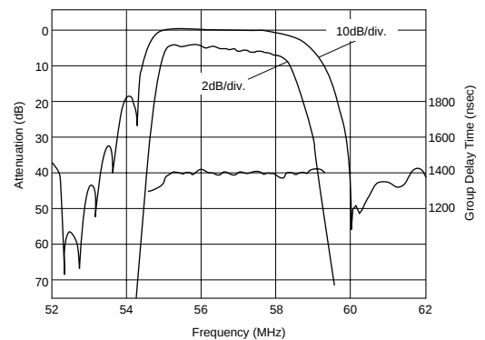
Frequency Characteristics
