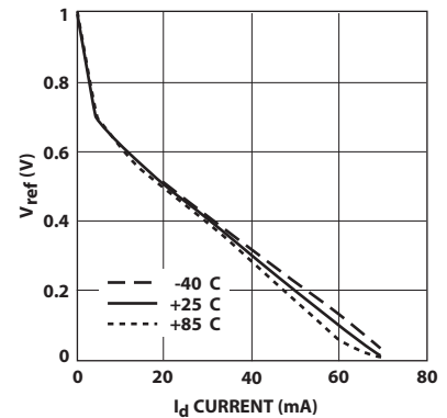
Figure 20. V_{ref} vs. Current and Temperature.
