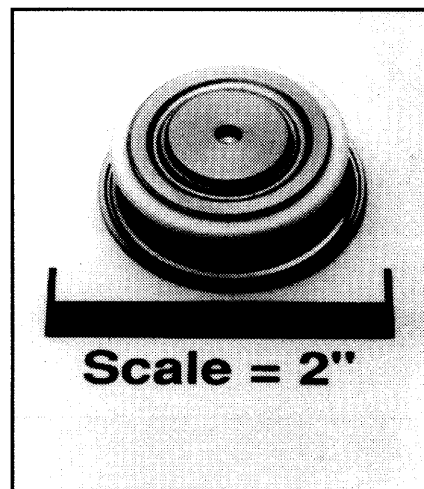
R620 General Purpose Rectifier 300-500 Amperes, 2400 Volts
