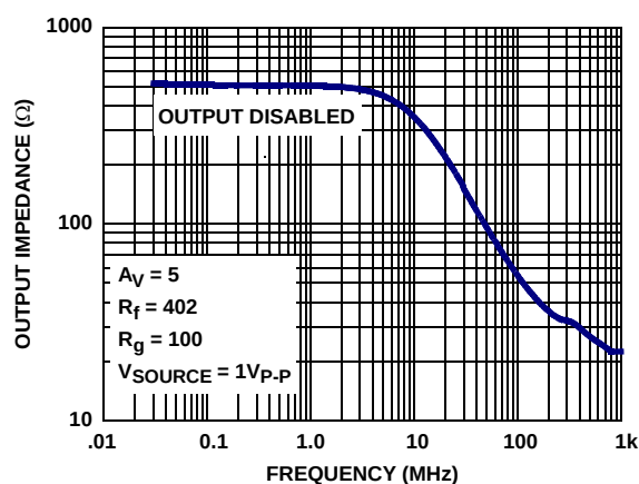
FIGURE 12. DISABLED OUTPUT IMPEDANCE vs FREQUENCY
