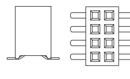
SMT Without Guide Post (S)
