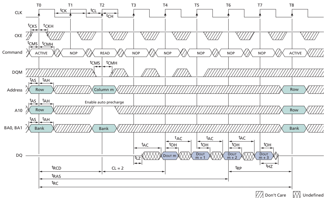
Figure 41: READ With Auto Precharge
