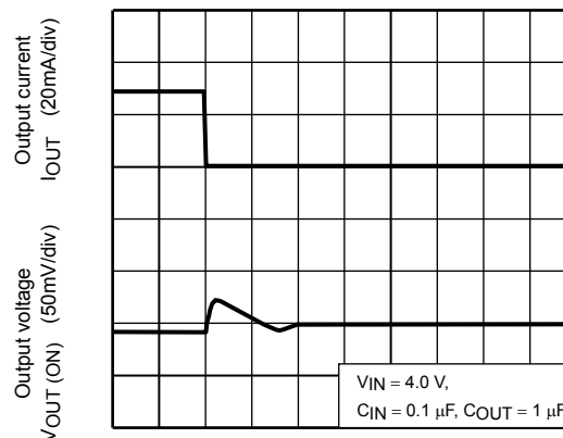
TCR5SB30A ( I_{OUT} = 30\text{m to } 1\text{mA} )
