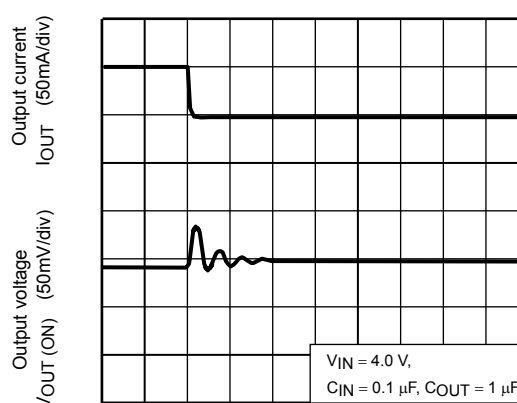
TCR5SB30A ( I_{OUT} = 100\text{m to } 50\text{mA} )
