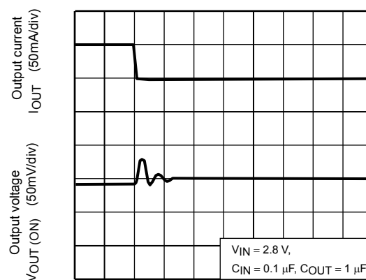
TCR5SB18A ( I_{OUT} = 100\text{m to } 50\text{mA} )
