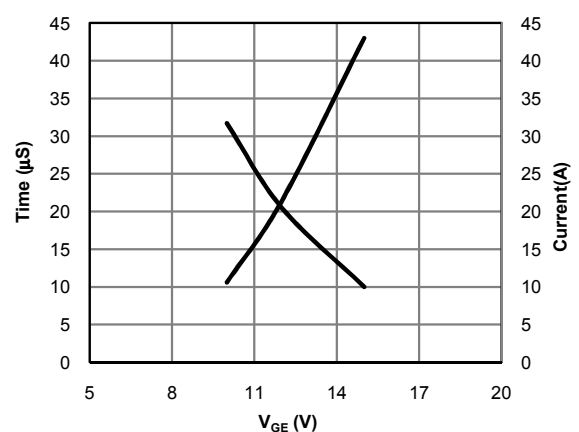
Fig 6: V_{GE} vs. Short Circuit Time ( V_{CE}=400\text{V}, T_j=25^{\circ}\text{C} )
